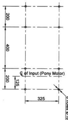
Layout of foundation bolt holes
