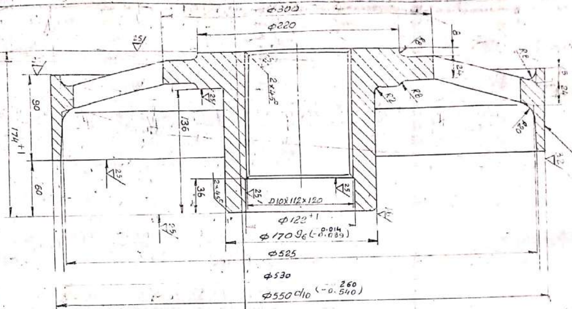
Detail I Scale - 2:1
