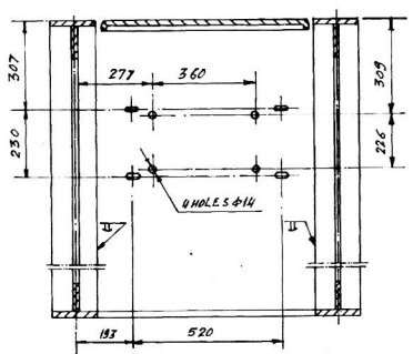
SECTION M-M
